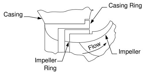
FIGURE 36. "L"-Type Wearing Ring
