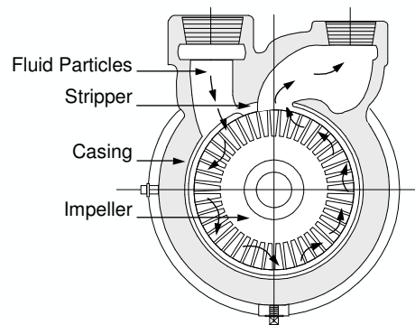
FIGURE 7. Turbine Pump
