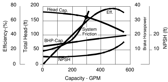
FIGURE 58. Pump Curve Superimposed over System Curve
