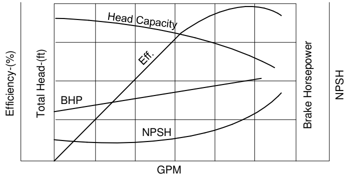
FIGURE 49. Overall Rating Curves
