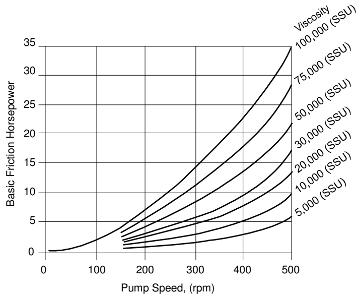
FIGURE 67. Effect of Viscosity Increase on Horsepower
