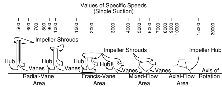
Figure 34. Impeller Profile vs. Specific Speed
