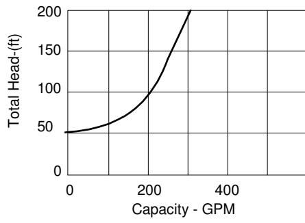
FIGURE 56. System Curve
