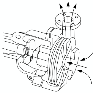
FIGURE 8. Viscous Drag Pump
