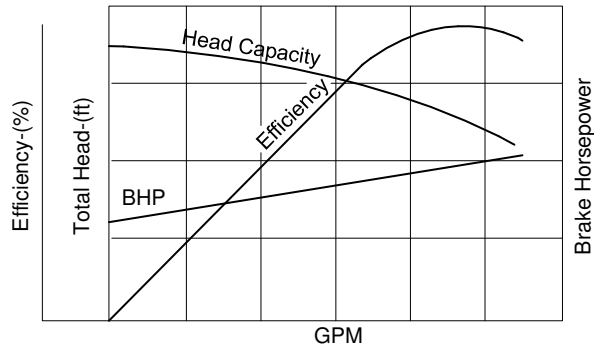
FIGURE 47. Efficiency-Capacity Curve
