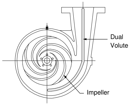
FIGURE 27. Volute Casing
