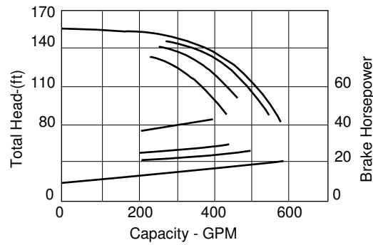
FIGURE 61. Effect of Viscosity Increase
