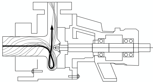
FIGURE 11. Vortex Pump
