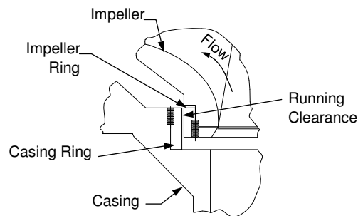
FIGURE 35. Flat-Type Wearing Ring
