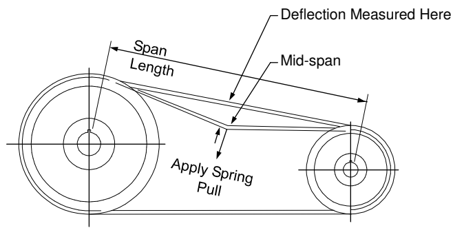
FIGURE 82. Correct Tension Check for V-belt Drives
