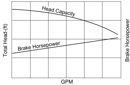
FIGURE 46. Brake-Horsepower-Capacity Curve
