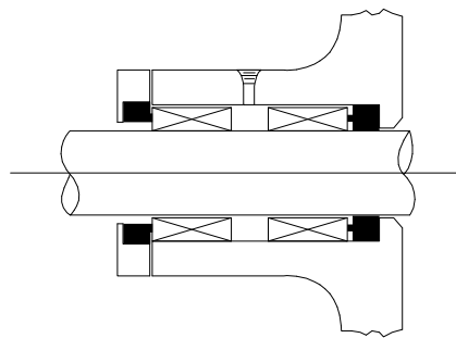
FIGURE 42. Double Seal
