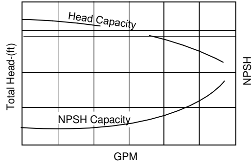
FIGURE 48. NPSH-Capacity Curve
