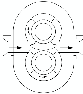
FIGURE 17. Circumferential, External Piston Pump
