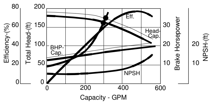
FIGURE 59. Effect of Variable Friction Loss
